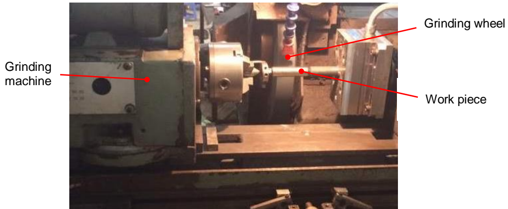
Figure 1. Experiment system
